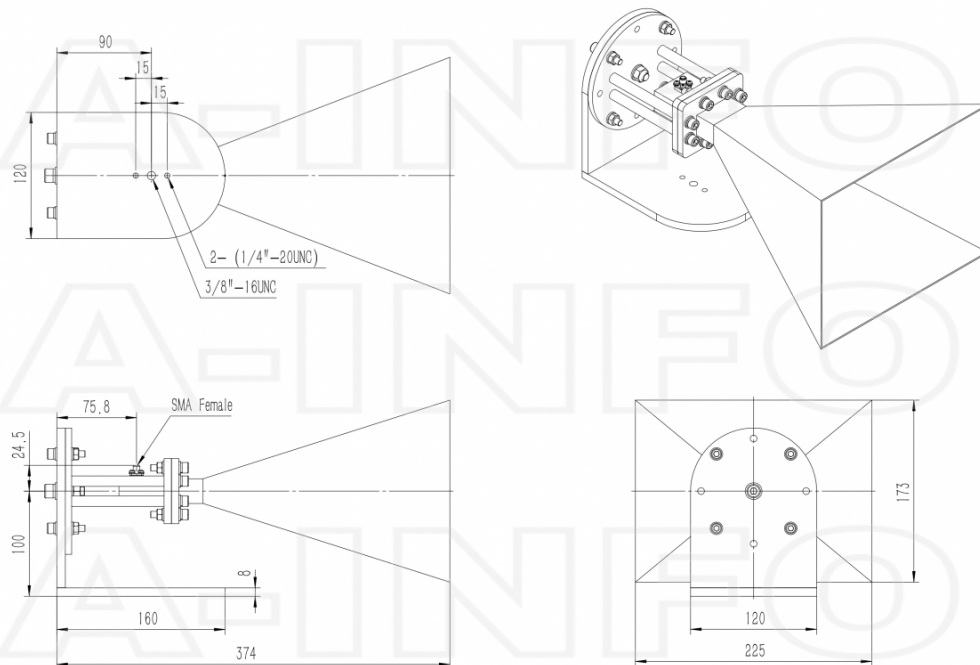
SMA Female Output with L Type Mounting Bracket (Option, P/N: LB-159-10-C-MBL)
