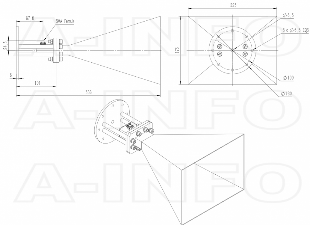
SMA Female Output with Round Mounting Bracket (Option, P/N: LB-159-10-C-MB)
