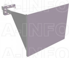
LB-159-20-C-SFSPO Standard Gain Horn Antenna 4.9-7.05GHz 20dB Gain SMA Female
